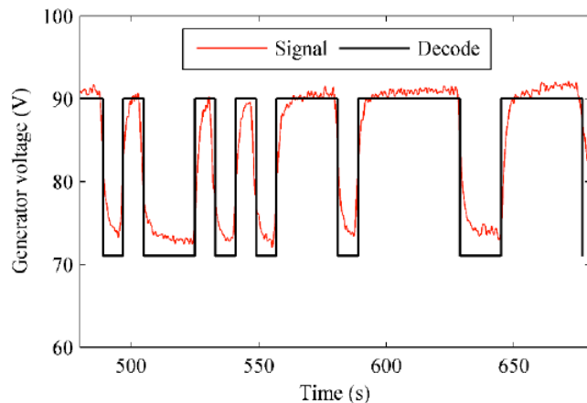
Figure 15: Decoding of downlink information under the pulse width of 8 seconds.
