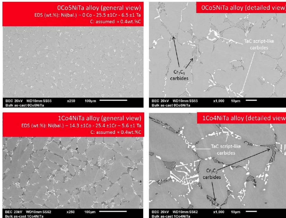
Figure 2: Microstructures of the two nickel-richer alloys in their as-cast states (top: 0Co5NiTa, bottom: 1Co4NiTa, left: \times 250 , right: \times 1000 ); left: composition measured by 5 full frame EDS on \times 250 areas.
