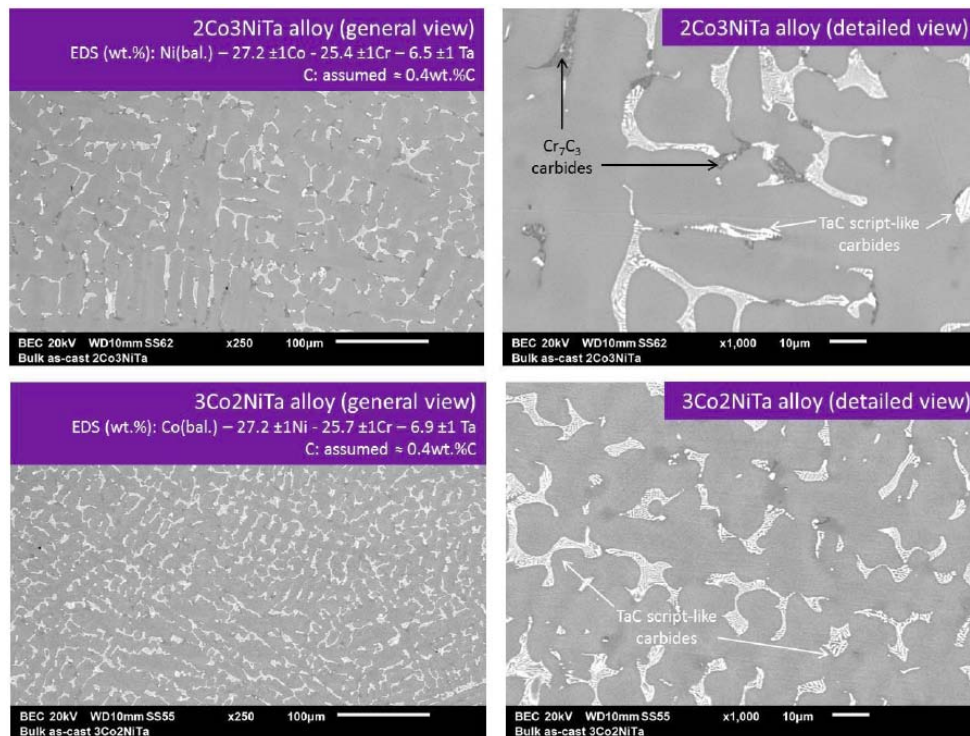
Figure 3: Microstructures of the two intermediate alloys in their as-cast states (top: 2Co3NiTa, bottom: 3Co2NiTa, left: \times 250 , right: \times 1000 ); left: composition measured by 5 full frame EDS on \times 250 areas.
